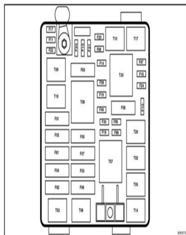
UNDERHOOD POWER DISTRIBUTION CENTER
